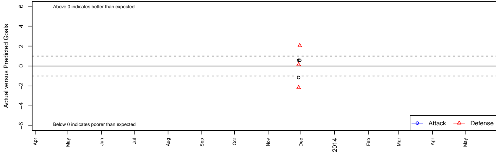
Surf Nike Select B01 Dots are actual minus expected GF (blue circles) and GA (red triangles). Blue line is smoothed change in attack strength. Red is smoothed change in defense strength.
